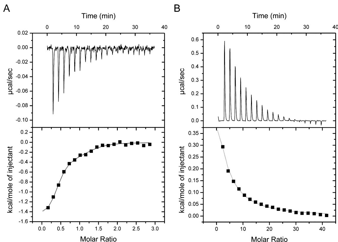
Figure 2. Isothermal titration calorimetry analysis of high- and low-affinity binding of \text{MgCl}_2 to PP2C \alpha . All titrations were performed at 25 °C. Bound metals were removed from purified PP2C \alpha by extensive dialysis against Chelex resin-treated buffers in the presence of excess Chelex resin. In each panel, the raw data are displayed in the upper figure, and the normalized, integrated injection heats are displayed in the lower panel. (A) Analysis of high-affinity sites with the titration of 550 \mu\text{M} \text{MgCl}_2 into 50 \mu\text{M} PP2C \alpha . The fitted curve is based on the two-site model. (B) Analysis of the low-affinity site with the titration of 30 mM \text{MgCl}_2 into 150 \mu\text{M} PP2C \alpha . The fitted curve is based on the one-site model.
