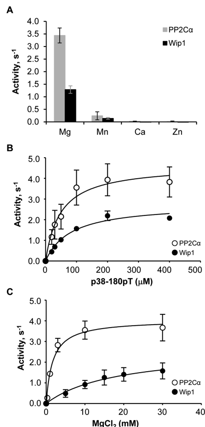
Figure 1. Substrate- and metal ion dependence of steady state phosphatase activity of human PP2C \alpha and Wip1. Activity assays were performed at 30 °C and contained 15 ng of purified PP2C \alpha or 60 ng of purified ProS2-Wip1(1–420). The initial rates were fitted to the Michaelis–Menten equation. Each point represents the average of at least three independent measurements. (A) Metal ion dependence of phosphatase activity. The activity was measured with 100 \mu M p38 \alpha (175–185)(180pT) peptide in the presence of 30 mM of the indicated chloride salts. (B) Phosphopeptide concentration dependence of phosphatase activity. The activity was measured with 0–400 \mu M p38 \alpha (175–185)(180pT) peptide in the presence of 30 mM MgCl 2 . (C) MgCl 2 concentration dependence of phosphatase activity. The activity was measured with 0.3–30 mM MgCl 2 in the presence of 100 \mu M p38 \alpha (175–185)(180pT) peptide.
