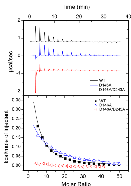
Figure 4. Isothermal titration calorimetry analysis of low-affinity binding of \text{MgCl}_2 to WT, D146A, and D146A/D243A PP2C \alpha proteins. Titrations were performed at 25 °C with 30 mM \text{MgCl}_2 titrated into 125–150 \mu\text{M} purified protein solution prepared by extensive dialysis against divalent ion-free buffer. Results shown are representative of two replicates. Upper panel: raw thermograms. The trace for PP2C \alpha is aligned to the axes; traces for the mutant proteins were shifted vertically for clarity. Lower panel: normalized, integrated injection heats, and the best-fit curve based on a one site binding model. The integrated heat of the first injection, which may be influenced by binding of \text{Mg}^{2+} ions to the high affinity sites, was not included in the fitting.
