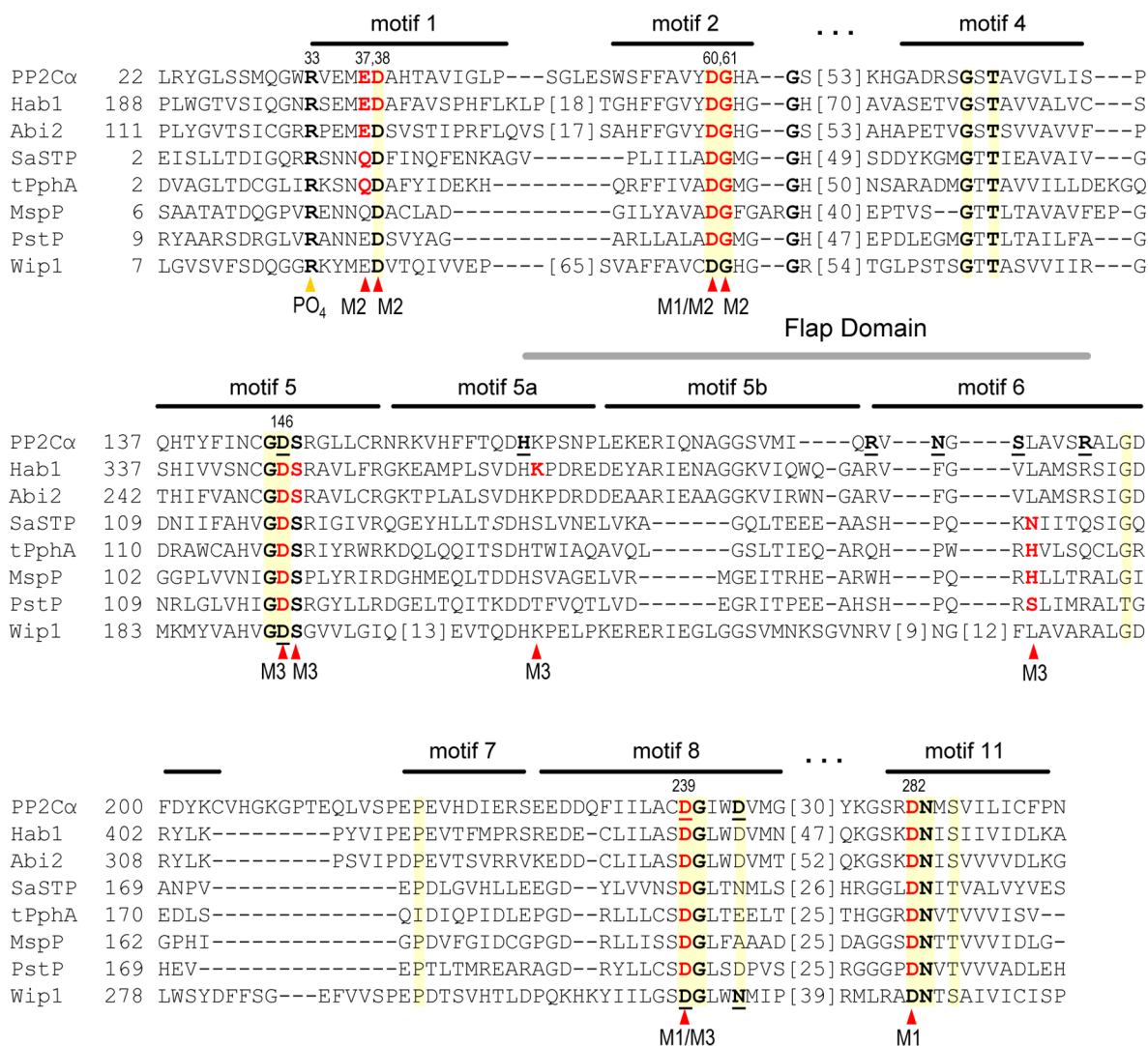
Figure 3. Multiple sequence alignment of human PP2Cα, Wip1, and several PP2C phosphatases displaying three active site metal ions. Alignment of catalytic domain sequences of seven structurally characterized PP2C phosphatases was performed using the program MUSCLE. 37 The Wip1 sequence was separately aligned. 38 Key residues are indicated by PP2Cα residue numbers. Metal ion-coordinating residues are indicated in red. The 15 previously identified highly conserved residues 4 are indicated by yellow shading. The Flap domain is indicated. Portions of the sequences were omitted for brevity. Mutated residues of PP2Cα and Wip1 discussed in this work are underlined and shown in bold.
