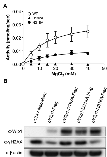
Figure 6. Mutation of putative third metal coordinating residues reduces or abolishes Wip1 phosphatase activity in vitro and in vivo. (A) MgCl_2 -concentration dependence of the in vitro phosphatase activity of wildtype and mutant Wip1. Phosphatase activity was measured at 30 °C using 100 \mu M p38 \alpha (175–185)(180pT) peptide in the presence of 0.3–40 mM MgCl_2 . Each point represents the average of at least three independent measurements. (B) \gamma H2AX level following exposure to IR reports phosphatase activity of WT or mutant Wip1 in vivo. To adjust the level of WT or Wip1 mutant proteins, HEK 293T cells were transfected with a constant total amount of DNA consisting of Wip1-Flag expression vector:parental vector in the following ratios: WT, 1:2; D192A, 1:2; D314A, 1:0.6; N318A, 1:0.2. Transfected cells were exposed to 10 Gy IR and were collected 90 min later. Isolated proteins were analyzed by Western blotting using antibodies specific for Wip1 and H2AX phosphorylated on Ser139 ( \gamma H2AX). \beta -Actin served as a loading control.
